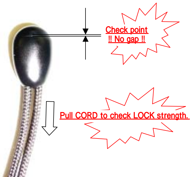
<pic-E> COMPLETION STATE
